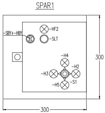
OUTLINE DIMENSIONS
