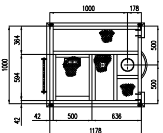
TORRETTA ROTANTE (TIPICA) ROTARY TURRET (TYPICAL)
