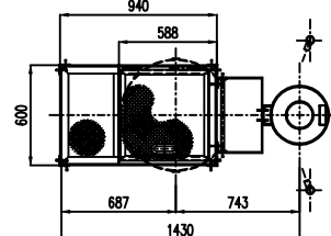
PIATTAFORMA INTERMEDIA (TIPICA) INTERMEDIATE PLATFORM (TYPICAL)
