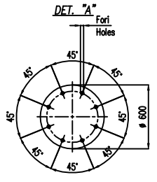
CONTROFLANGIA MASK PLATE Ø 600 thk. 10
